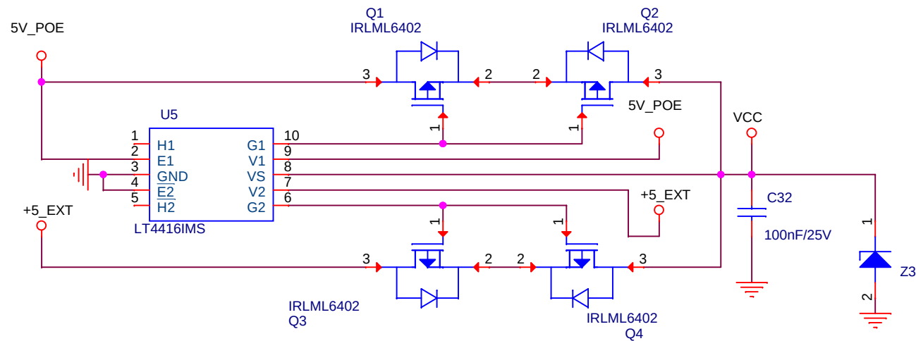
automatic power switch
