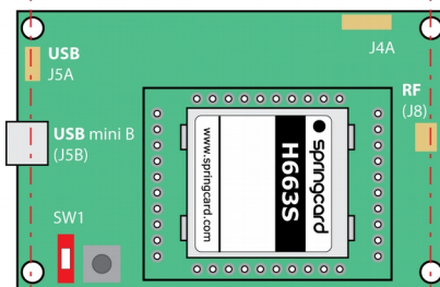
EN Main board top view
