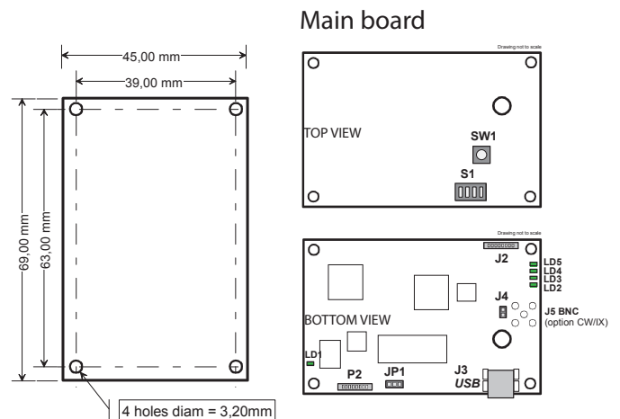
Same outside dimensions for the 2 boards thickness = 1,6 mm - global tolerance = ± 0,1 mm
